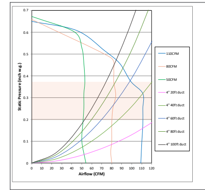
FV-0511VHL1 110 CFM 4" Duct
