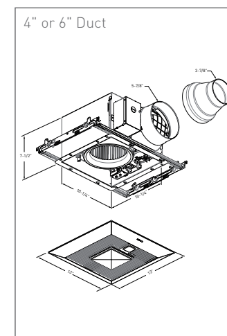
FV-0511VKSL3
