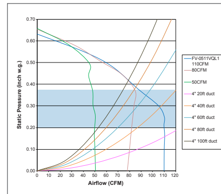
FV-0511VQL1 50-80-110 CFM 4" or 6" Duct
