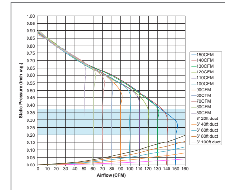
FV-15NLF51H 50-150 CFM 6" Duct
