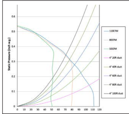
FV-0511VFL1 - 4" Duct
