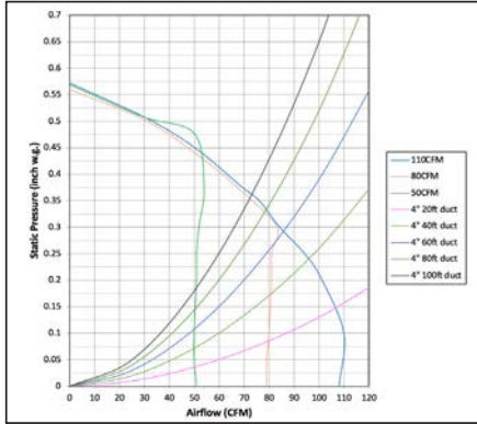
FV-0511VFC1 - 4" Duct
