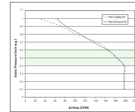
FV-20VEC1 200 CFM 6" Ducts
