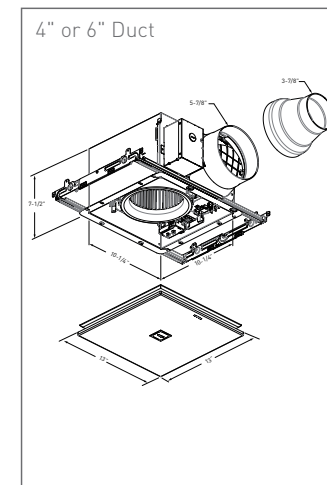
FV-0511VKS3S
