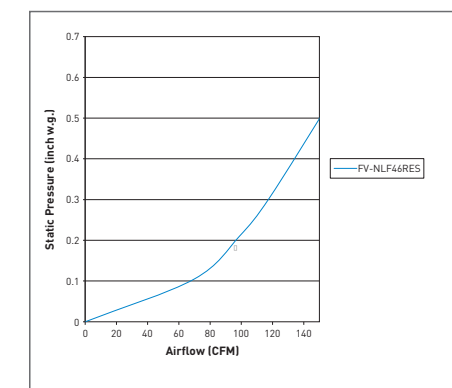
FV-NLF46RES 4" or 6" Duct*
