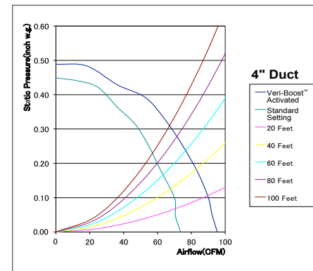
FV-07VBA1A + FV-07VBB1 4" Ducts
