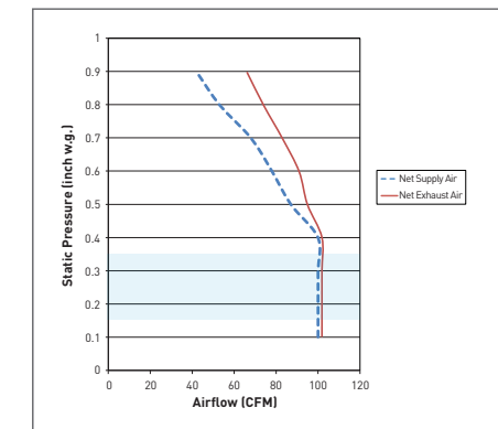
Intelli-Balance 100 Airflow Performance Curve 4 or 6" Ducts
