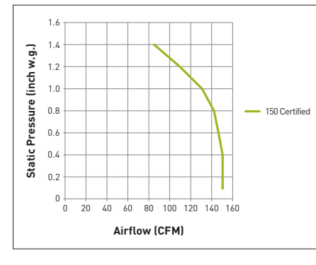
FV-15VE1S Net Supply
