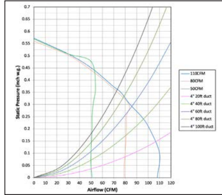
FV-0511VF1 - 4" Duct
