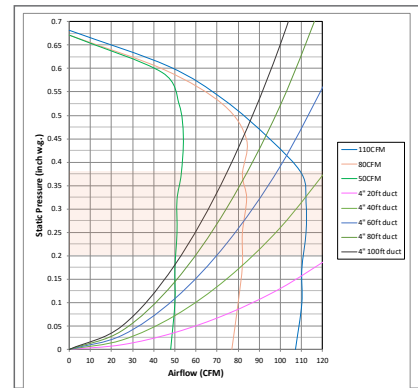
FV-0511VH1 110 CFM 4" Duct
