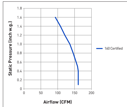
FV-13VEC1S Net Supply
