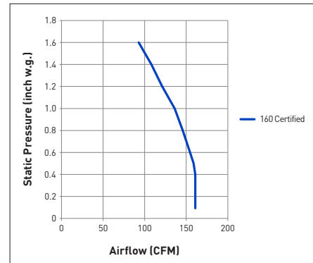
FV-15VE1T Net Supply
